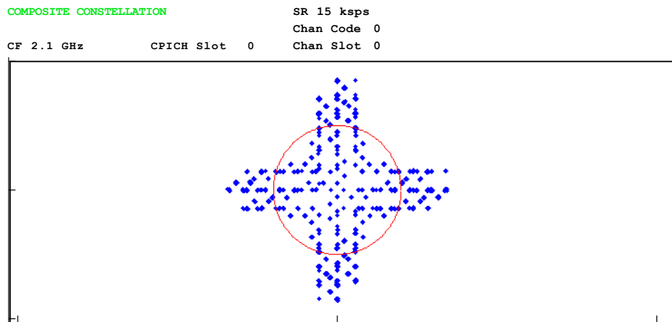
Bild 26 Composite Constellation diagram of received signal (scrambled chips)
